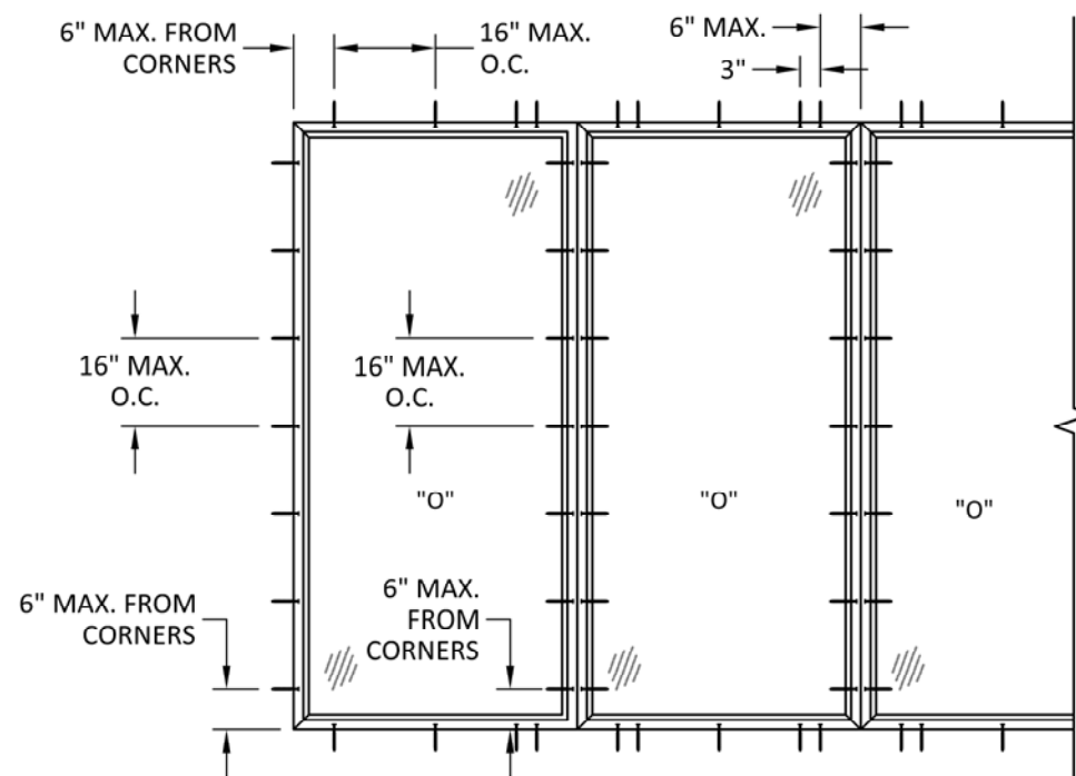
ANCHOR LAYOUT MULLED - THROUGH FRAME - FIXED WINDOW
